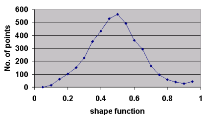
Fig. 1. Histogram of shape function values for the trypsin molecule (PDB code 2ptn).
